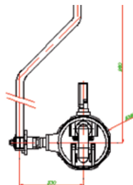
Electric drive
